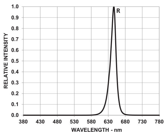
Figure 1: Relative Luminous Intensity vs. Wavelength
