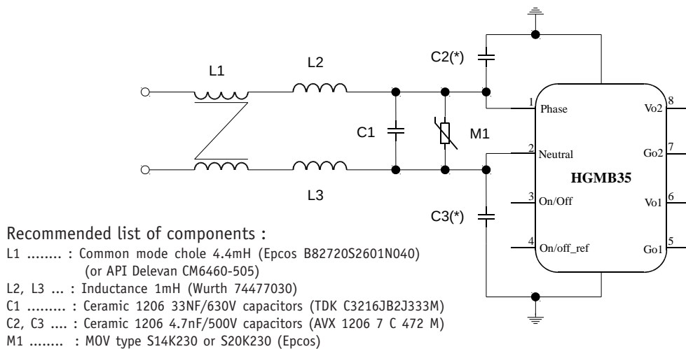
Fig : D0-160D Conducted Noise Emission
